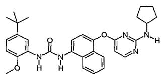
1-(5-tert-Butyl-2-methoxy-phenyl)-3-[4-(2-cyclopentylamino-pyrimidin-4-yloxy)-naphthalen-1-yl]-urea;
